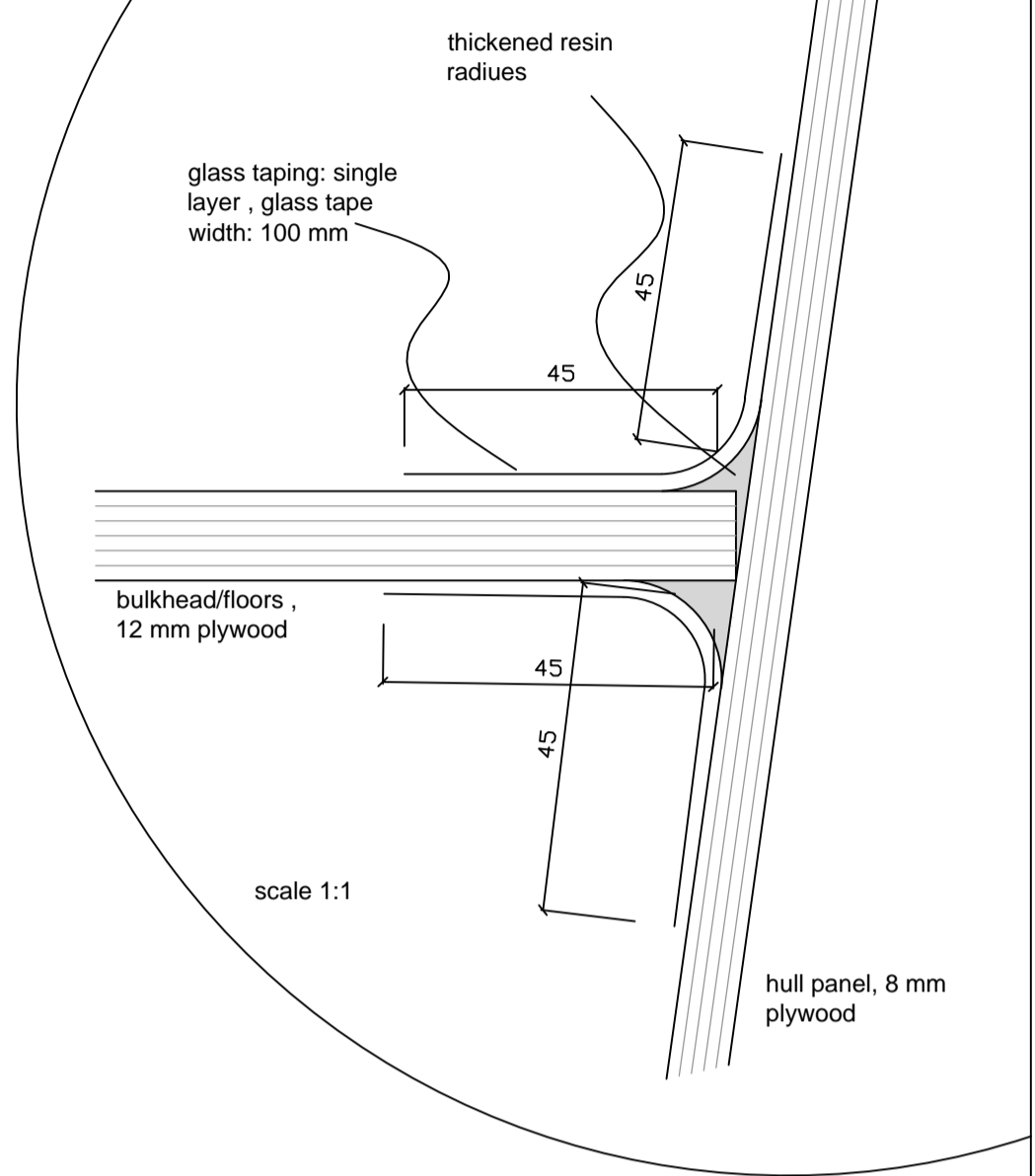
typical hull panels-bulkhead/floors joint detail
